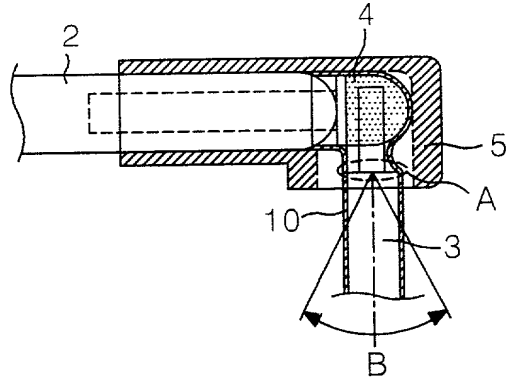
FIG. 3 CONVENTIONAL ART
